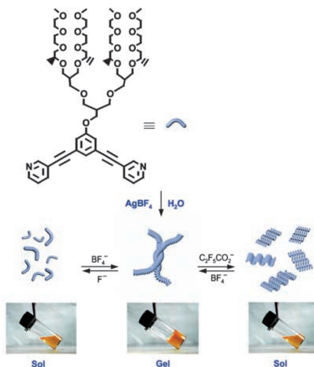
Figure 1. Schematic representation of reversible polymerization and reversible conversion between folded and unfolded conformations of a coordination chain upon counteranion exchange.
