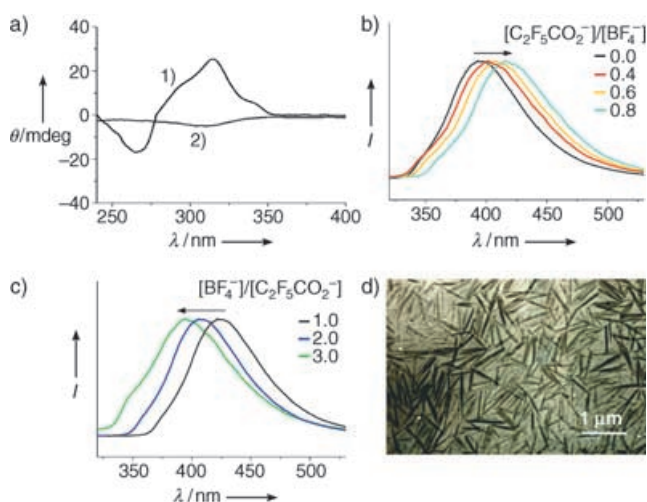
Figure 3. a) Circular dichroism (CD) spectra of: 1) [\text{Ag-2}]\text{BF}_4 (5 wt %); 2) [\text{Ag-2}]\text{BF}_4 (5 wt %) after the addition of 1 equiv \text{Bu}_4\text{N}^+\text{C}_2\text{F}_5\text{CO}_2^- . b) Fluorescence spectra of [\text{Ag-2}]\text{BF}_4 (5 wt %) with increasing amounts of \text{Bu}_4\text{N}^+\text{C}_2\text{F}_5\text{CO}_2^- . c) Fluorescence spectra of a mixture of [\text{Ag-2}]\text{BF}_4 (5 wt %) and \text{Bu}_4\text{N}^+\text{C}_2\text{F}_5\text{CO}_2^- (1:1) with increasing amounts of \text{Bu}_4\text{N}^+\text{BF}_4^- . d) TEM image of [\text{Ag-2}]\text{C}_2\text{F}_5\text{CO}_2 in \text{H}_2\text{O} (0.3 wt %) stained with \text{RuO}_4 .
