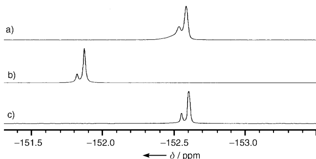
Figure 4. Comparison of ^{19}\text{F} NMR spectra in \text{D}_2\text{O} (470 MHz, 298 K): a) free \text{AgBF}_4 ; b) [\text{Ag-2}]\text{BF}_4 (5 wt %); c) [\text{Ag-2}]\text{BF}_4 (5 wt %) after the addition of 1 equiv of \text{Bu}_4\text{N}^+\text{C}_2\text{F}_5\text{CO}_2^- . The chemical shifts were measured as upfield shifts relative to that of \text{CFCl}_3 as an external standard.
