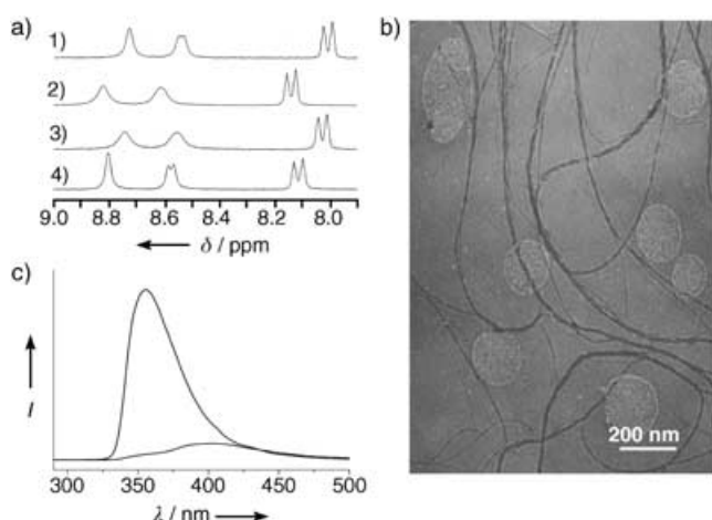
Figure 2. a) ^1\text{H} NMR spectra (250 MHz, 298 K) in \text{CD}_3\text{OD} (1 wt %) of 1) 2; 2) [\text{Ag-2}]\text{BF}_4 ; 3) [\text{Ag-2}]\text{BF}_4 and 1.2 equiv \text{Bu}_4\text{N}^+\text{F}^- ; 4) same as (3) after the addition of 1.2 equiv \text{Bu}_4\text{N}^+\text{BF}_4^- . b) TEM image of dried gel from [\text{Ag-2}]\text{BF}_4 in \text{H}_2\text{O} (0.3 wt %) stained with \text{RuO}_4 . c) Fluorescence spectra of 2 and gel of [\text{Ag-2}]\text{BF}_4 (5 wt % in \text{H}_2\text{O} ; \lambda_{\text{ex}} = 275 nm).
